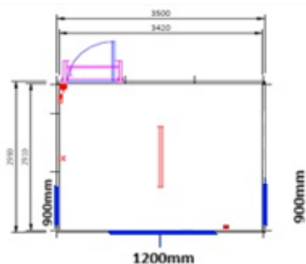
fig 1. Floor plan
