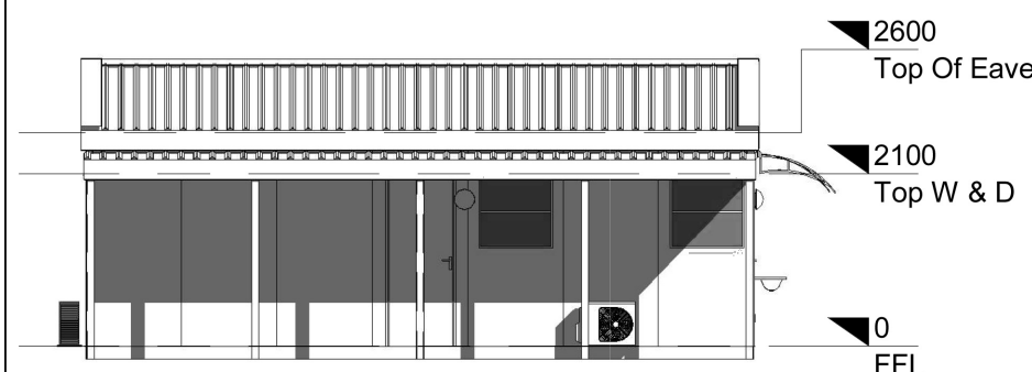
2 South Elevation
