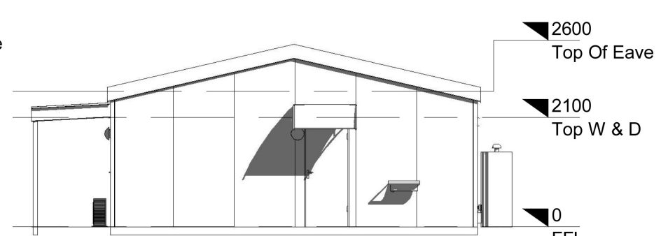
3 East Elevation
