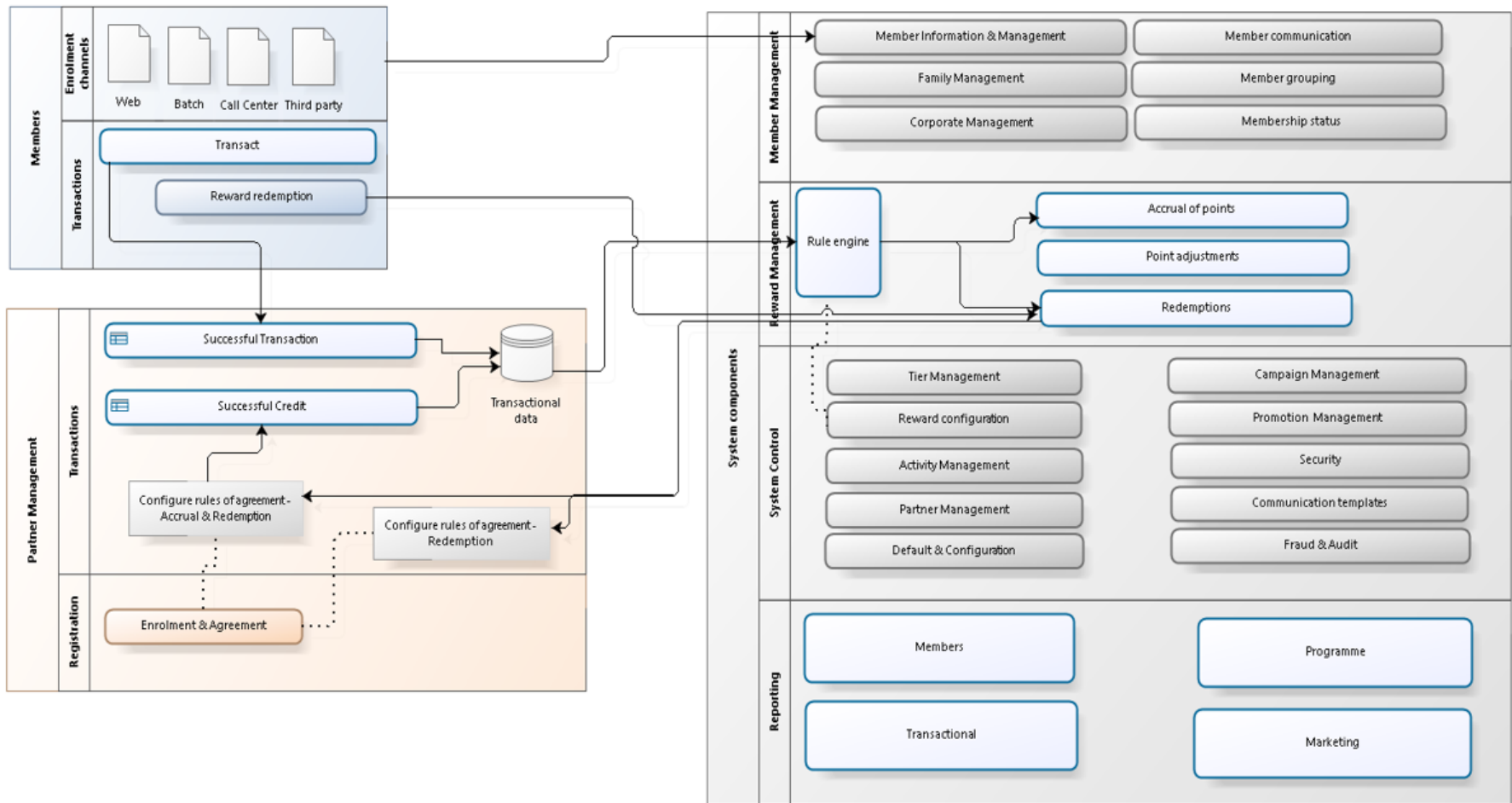
• Figure 1 - Schematic representation of the relevant components of the LoyaltyPlus software solution
