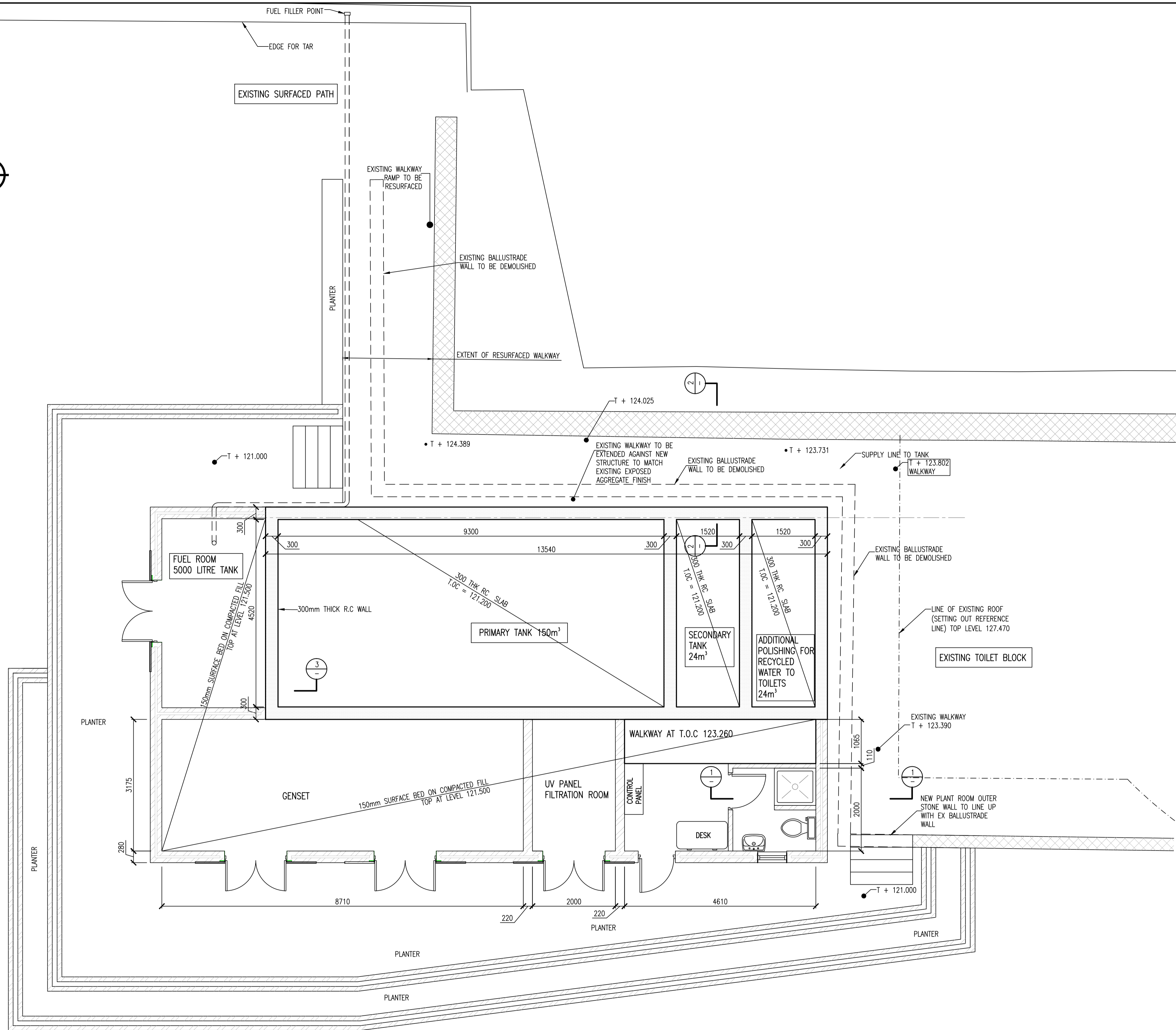
1:50 GROUND LEVEL LAYOUT
