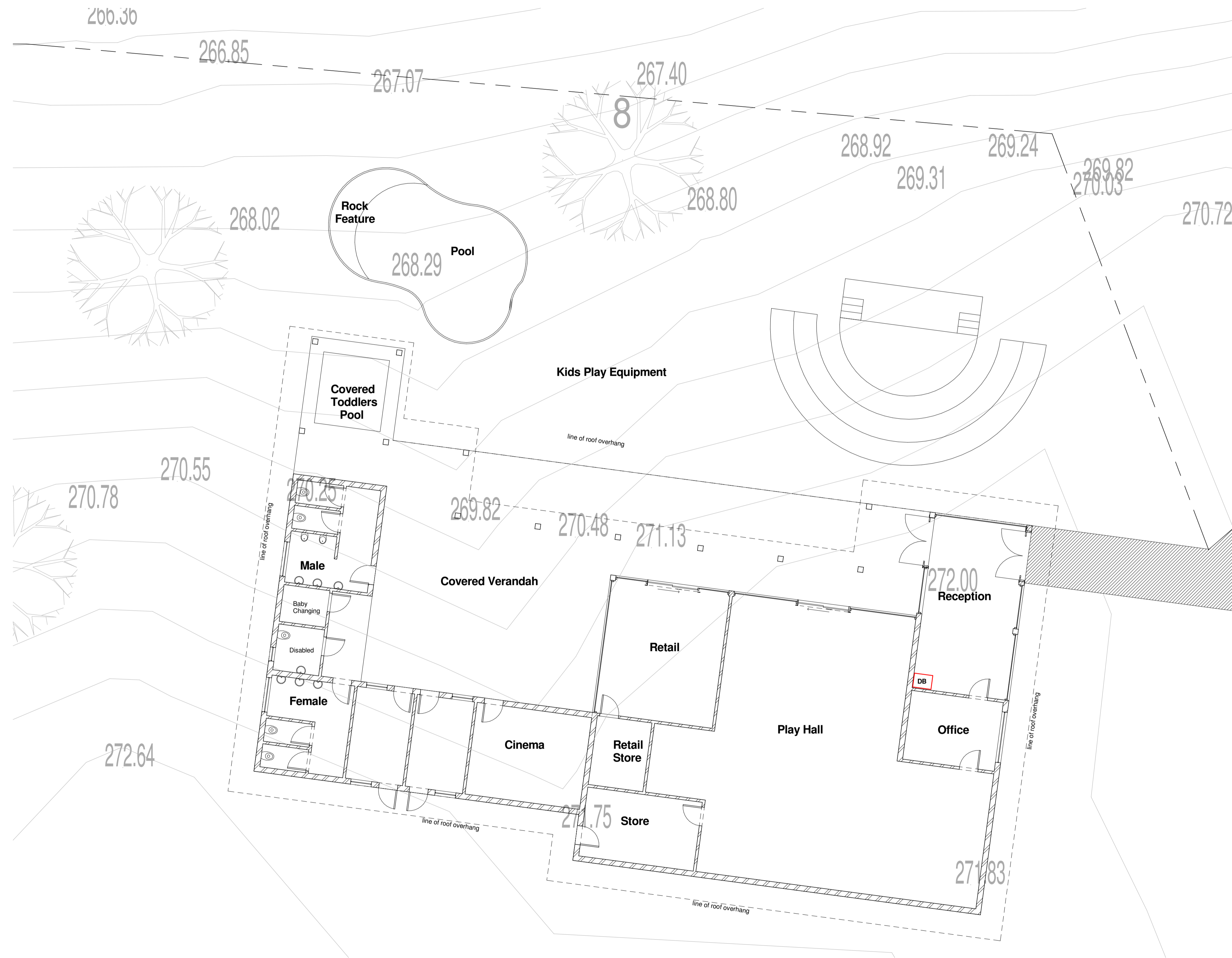
1 Ground Floor Plan 1 : 100
